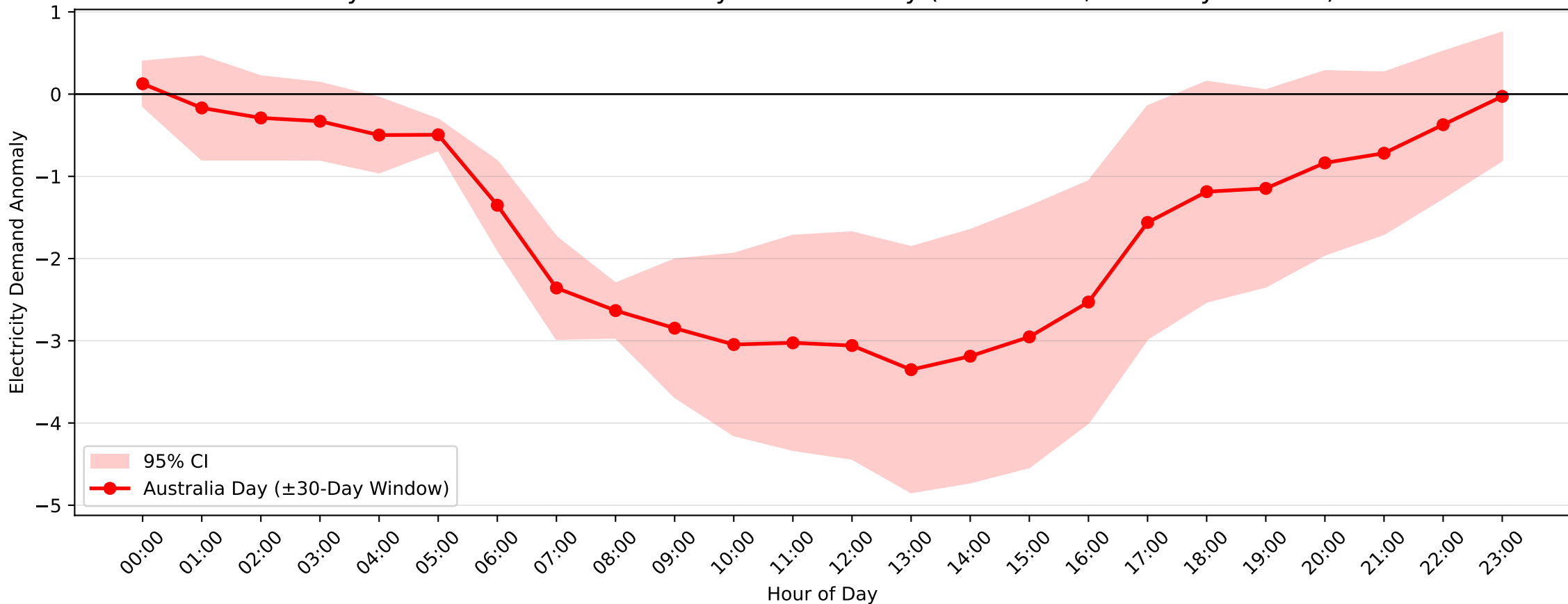
Mayfield West Demand Anomaly: Australia Day (2004-2017, \pm 30 -Day Window)
